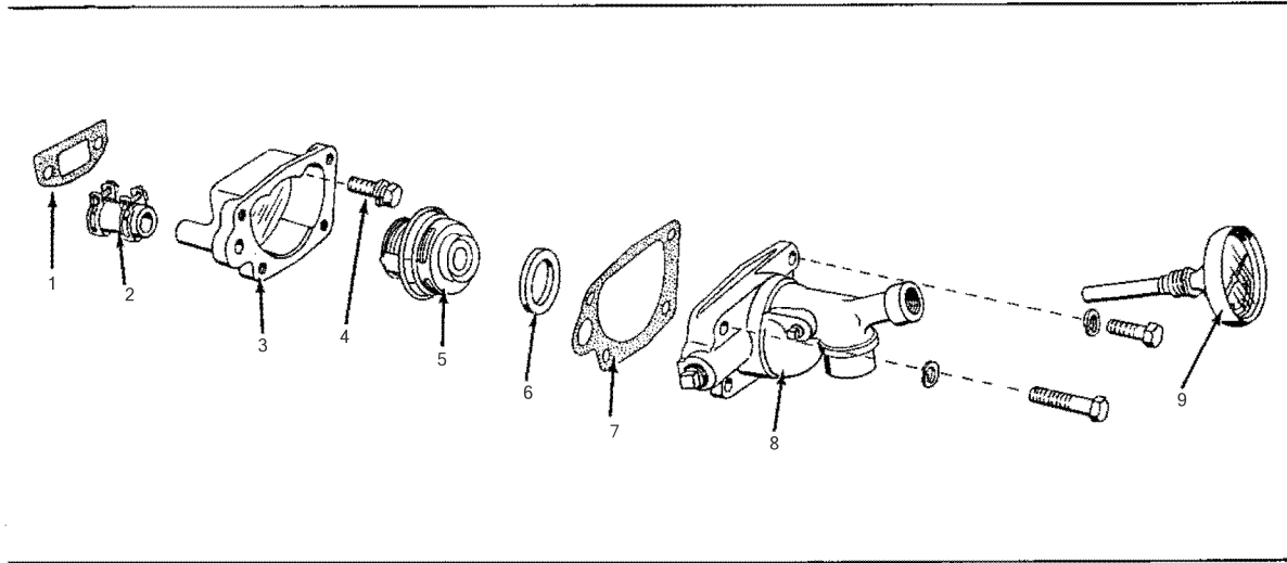
WATER MANIFOLD BY-PASS
